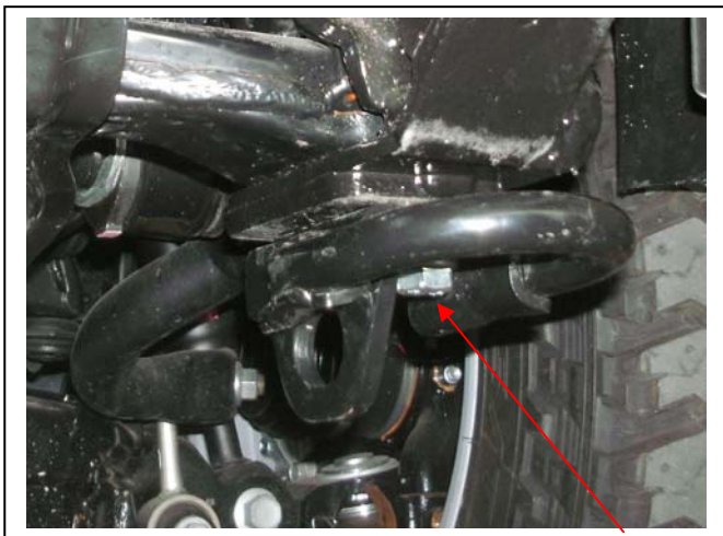
Figure 5: Bolts through tow hook assemblies
